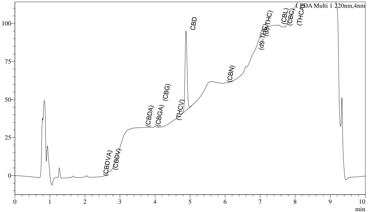
Chromatogram
